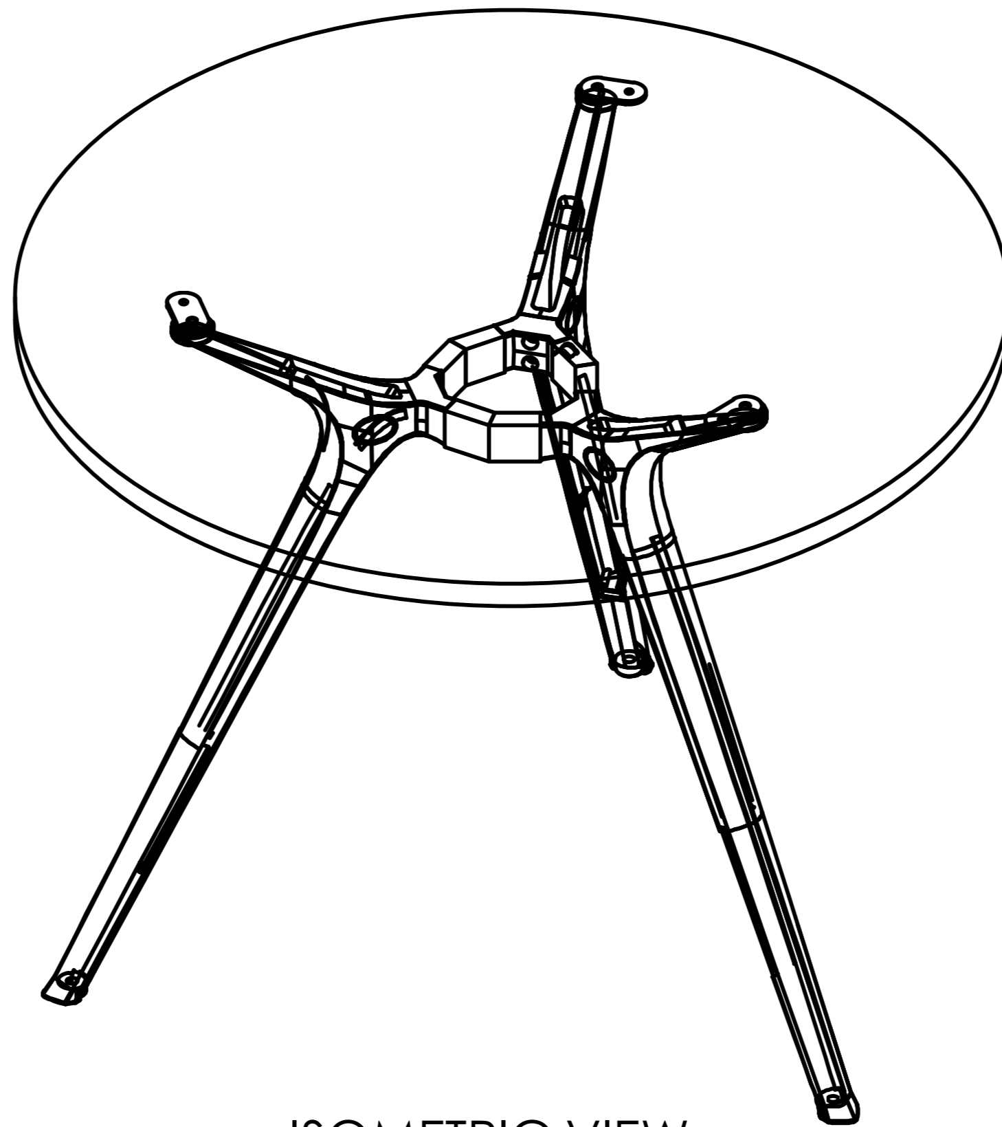
ISOMETRIC VIEW
