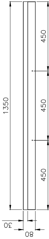
TOP VIEW
