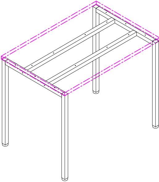
ISOMETRIC VIEW
