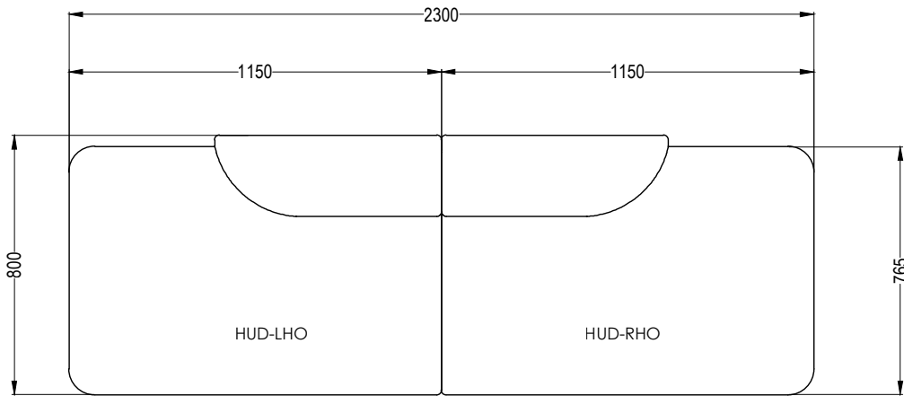
TOP VIEW
