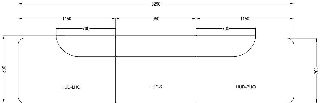
TOP VIEW
