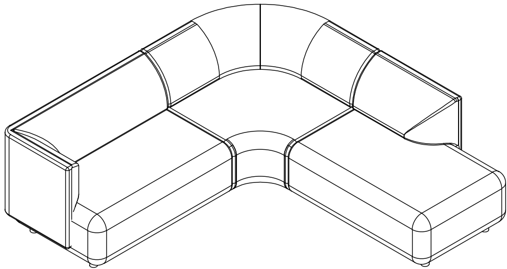
ISOMETRIC VIEW
