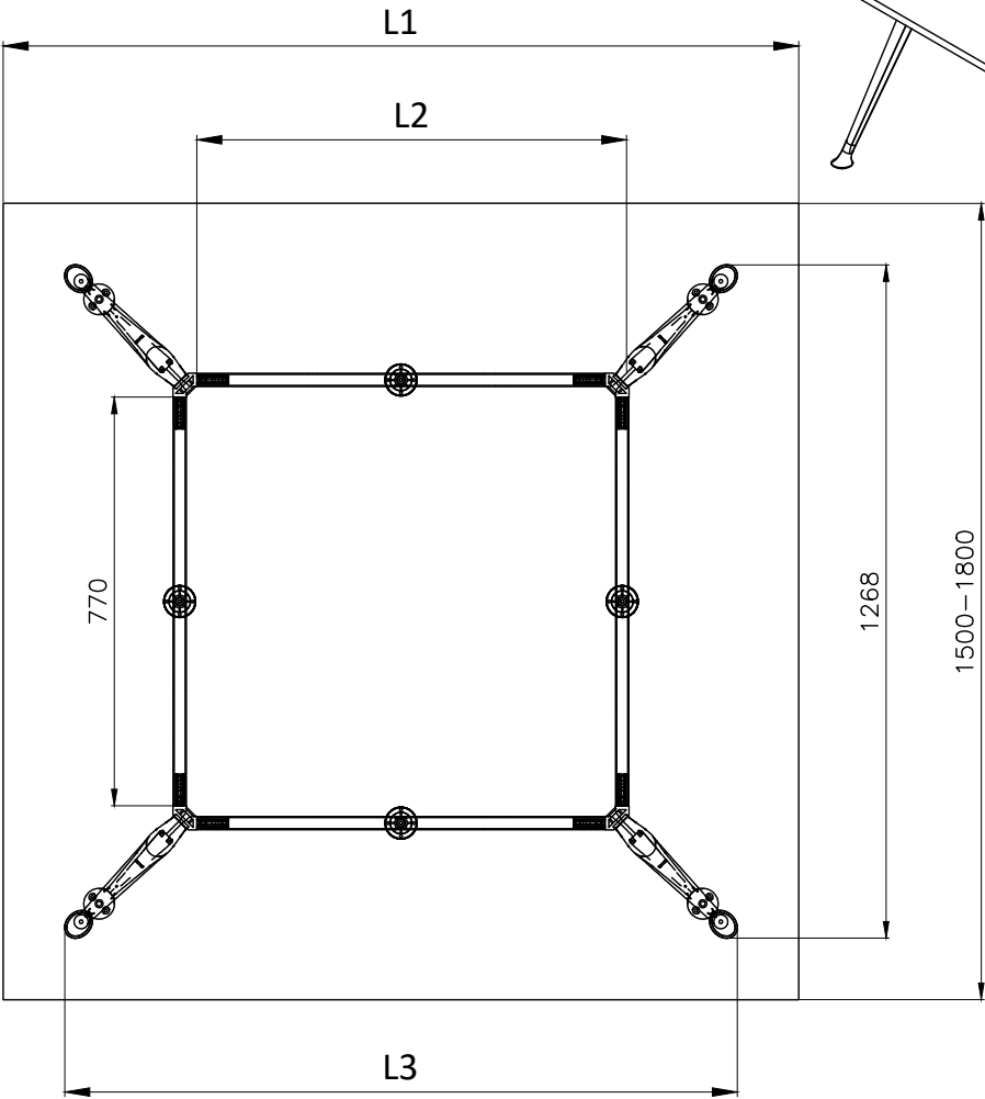
TOP VIEW
