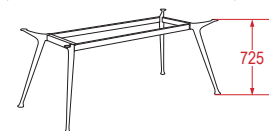
K2-1890 725mm High 4 Leg Frame Suits 1800mm x 900mm Top
