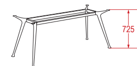
K2-1875 725mm High 4 Leg Frame Suits 1800mm x 750mm Top
