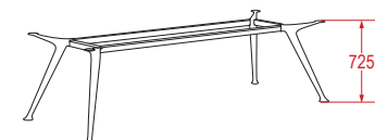
K2-2475 725mm High 4 Leg Frame Suits 2400mm x 750mm Top
