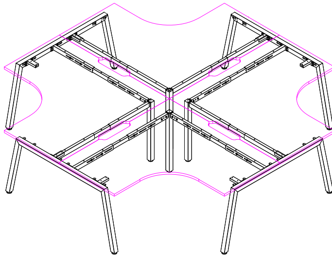
ISOMETRIC
