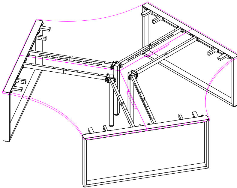
ISOMETRIC VIEW
