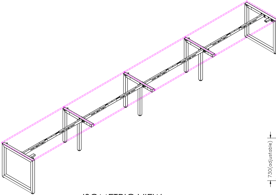
ISOMETRIC VIEW
