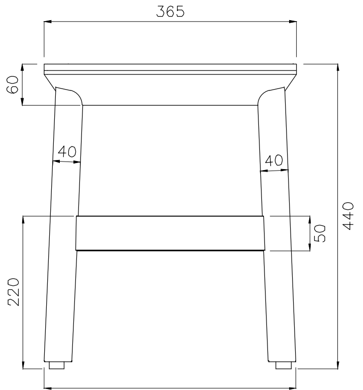
SIDE VIEW
