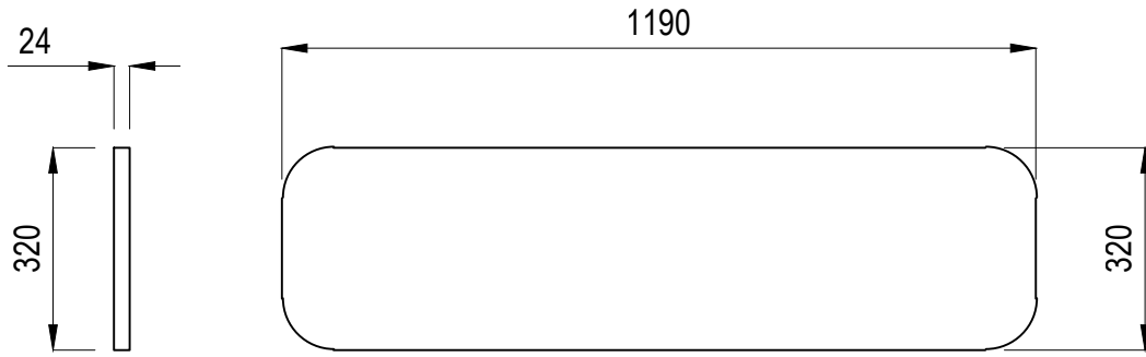
1190 x 320 x 24mm HY-DT24-1190/LG HY-DT24-1190/CF
